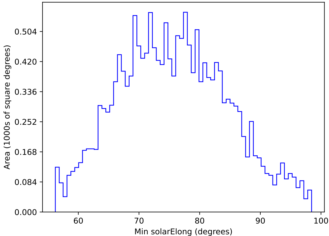
internal_u_expt30_nscale1.0v3.4_10yrs WFD g band: Min solarElong
