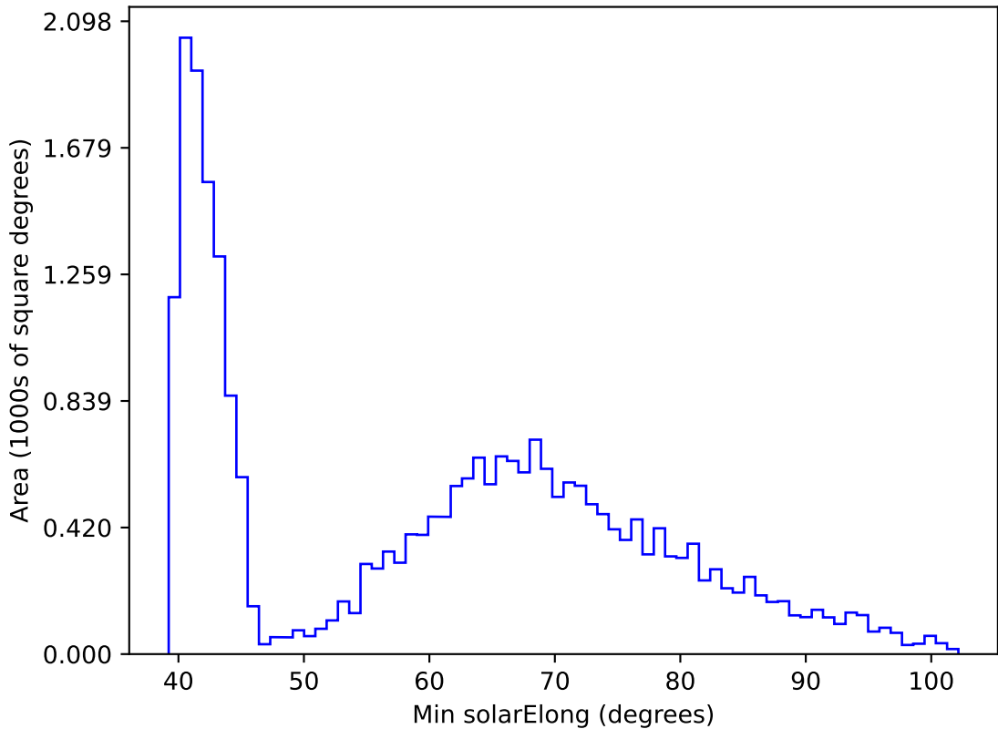
internal_u_expt30_nscale1.0v3.4_10yrs All sky r band: Min solarElong
