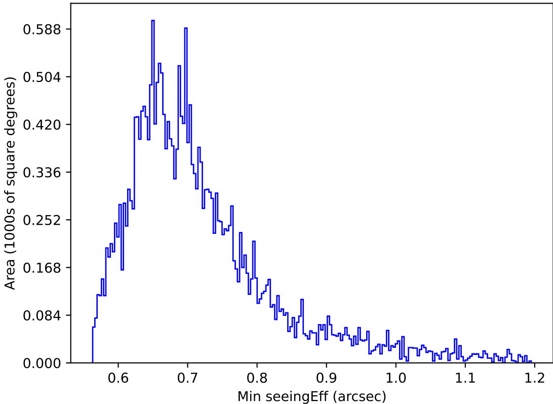
internal_u_expt30_nscale1.0v3.4_10yrs Yr 1 z band: Min seeingEff
