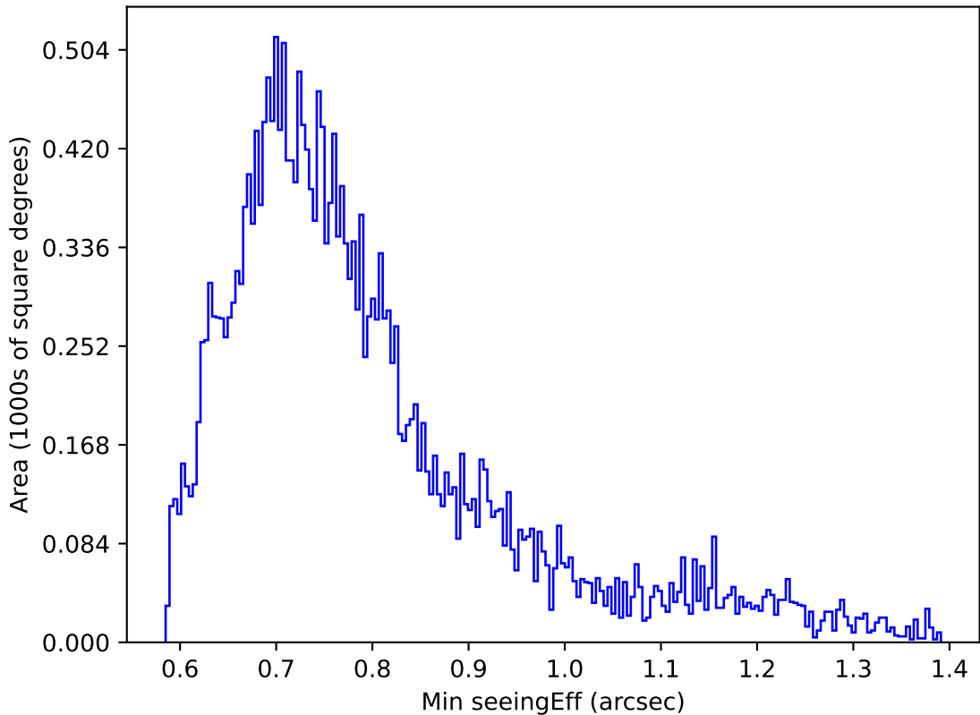
internal_u_expt30_nscale1.0v3.4_10yrs Yr 1 g band: Min seeingEff
