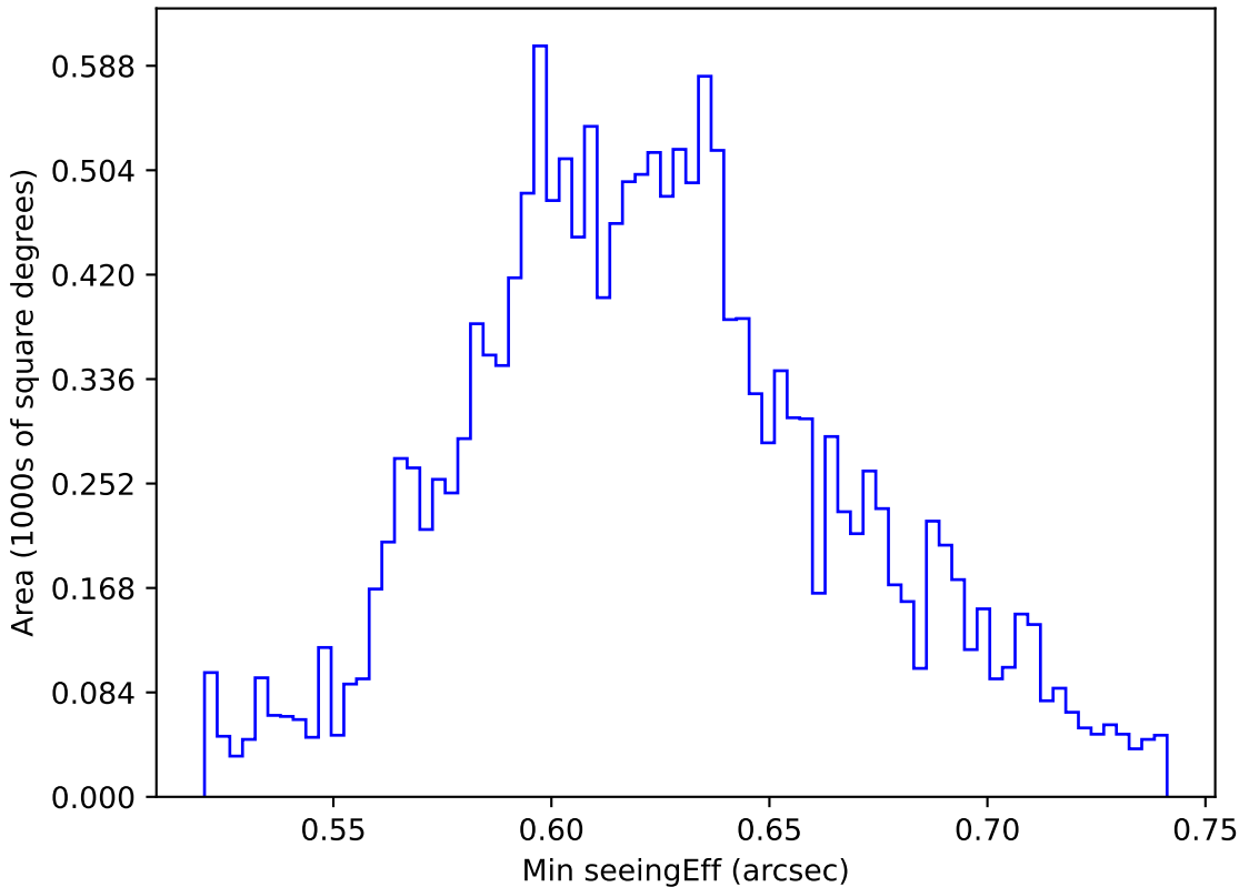
internal_u_expt30_nscale1.0v3.4_10yrs WFD y band: Min seeingEff
