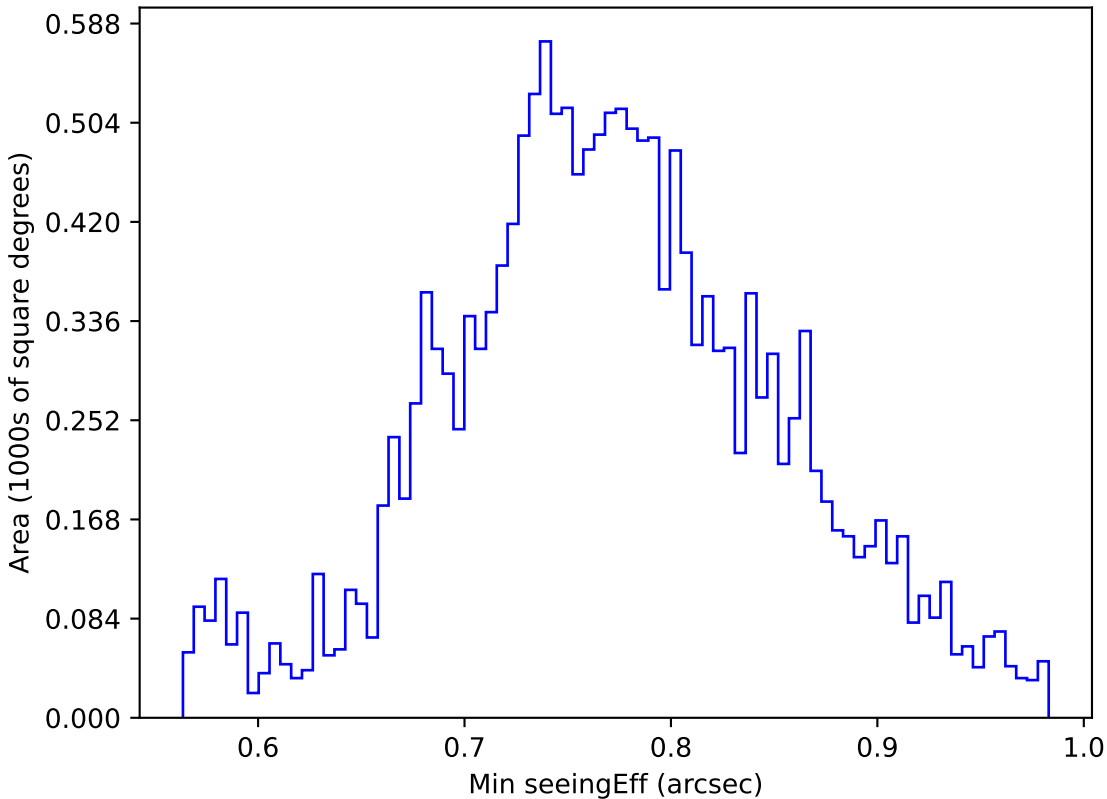
internal_u_expt30_nscale1.0v3.4_10yrs WFD u band: Min seeingEff
