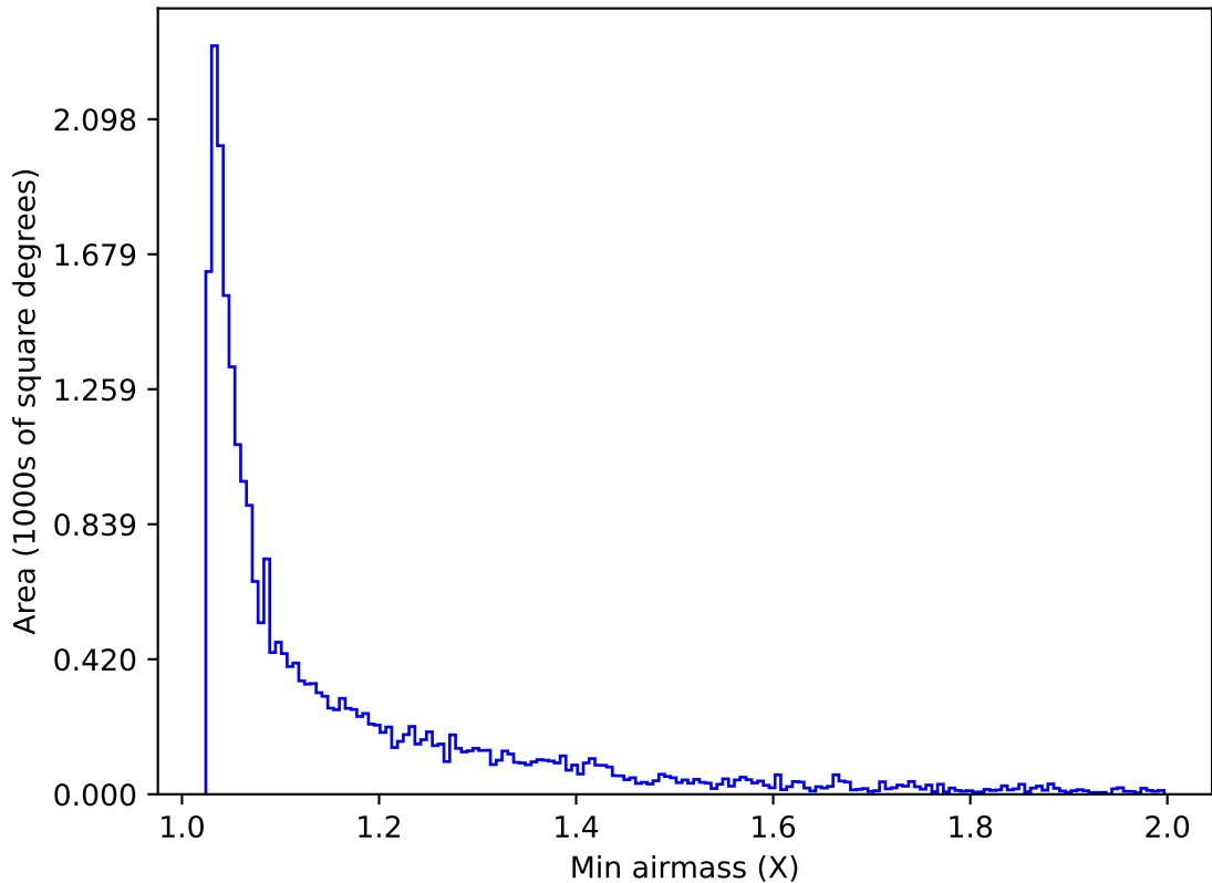
internal_u_expt30_nscale1.0v3.4_10yrs Yr 1 z band: Min airmass
