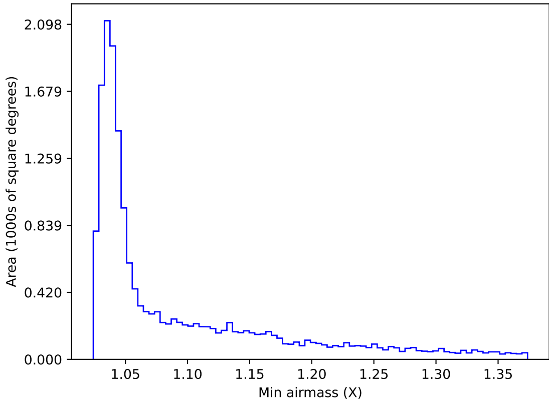
internal_u_expt30_nscale1.0v3.4_10yrs WFD u band: Min airmass
