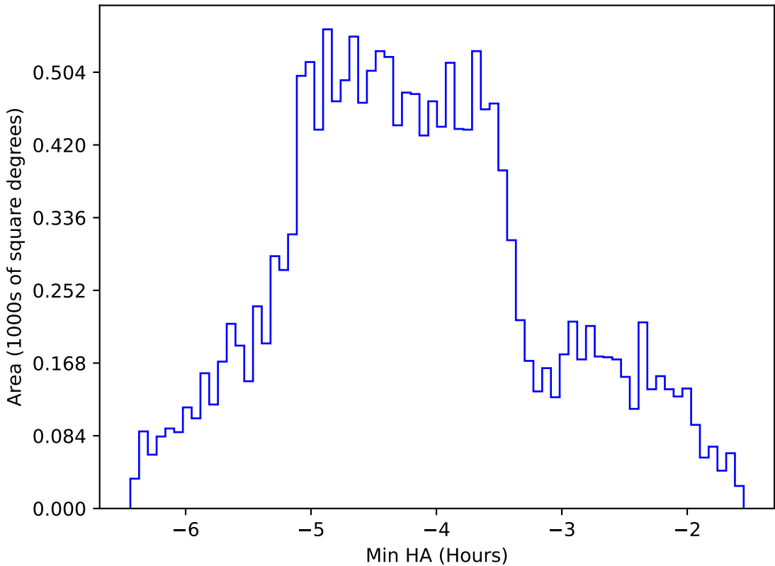
internal_u_expt30_nscale1.0v3.4_10yrs WFD g band: Min HA
