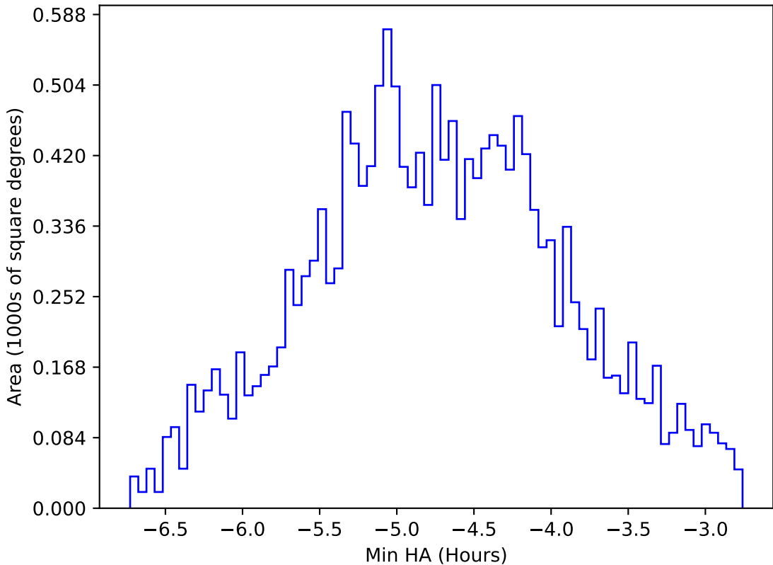
internal_u_expt30_nscale1.0v3.4_10yrs WFD all bands: Min HA
