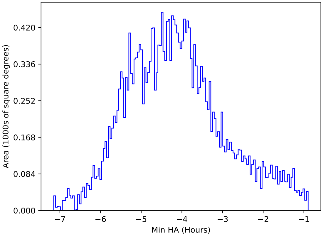
internal_u_expt30_nscale1.0v3.4_10yrs All sky r band: Min HA
