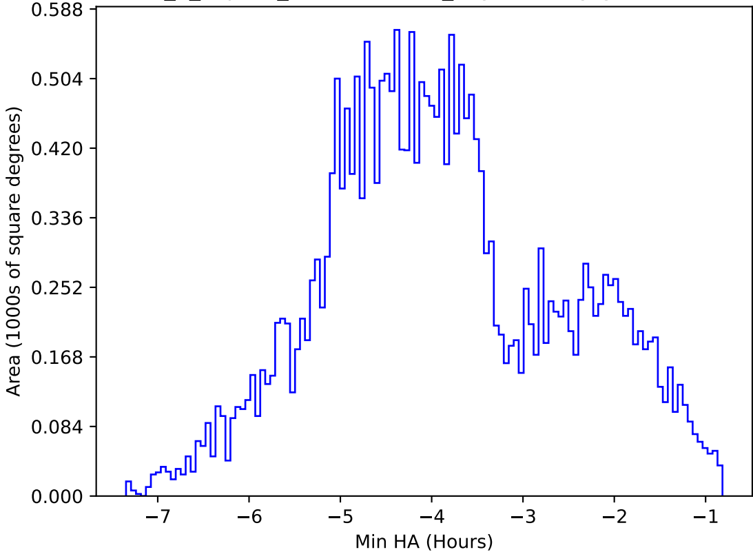
internal_u_expt30_nscale1.0v3.4_10yrs All sky g band: Min HA
