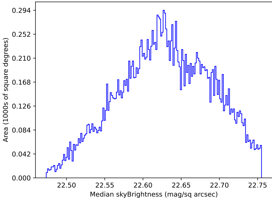
internal_u_expt30_nscale1.0v3.4_10yrs Yr 1 u band: Median skyBrightness
