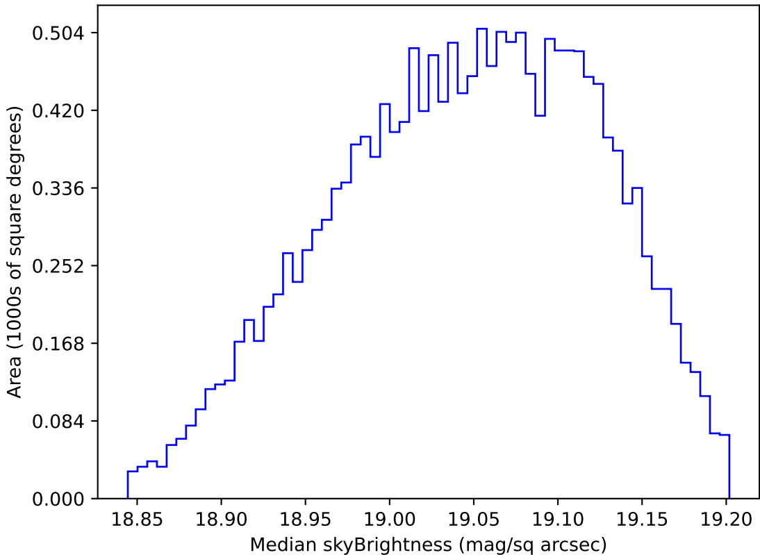
internal_u_expt30_nscale1.0v3.4_10yrs WFD z band: Median skyBrightness
