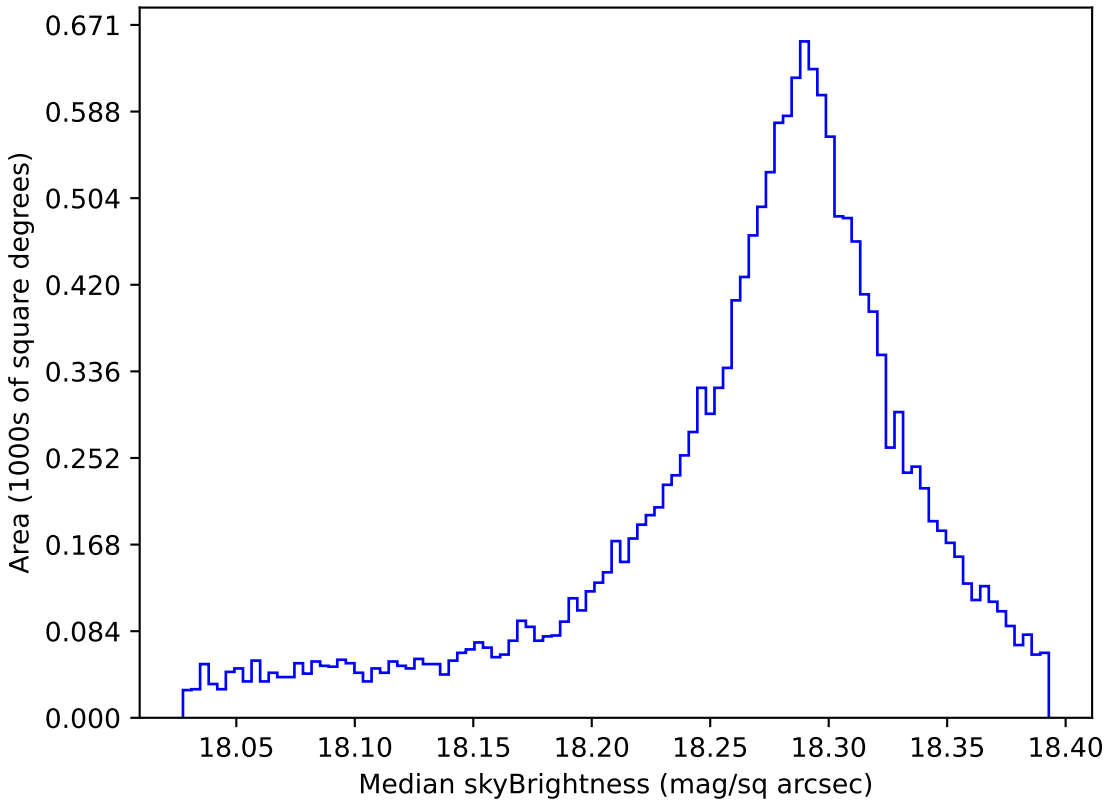
internal_u_expt30_nscale1.0v3.4_10yrs WFD y band: Median skyBrightness
