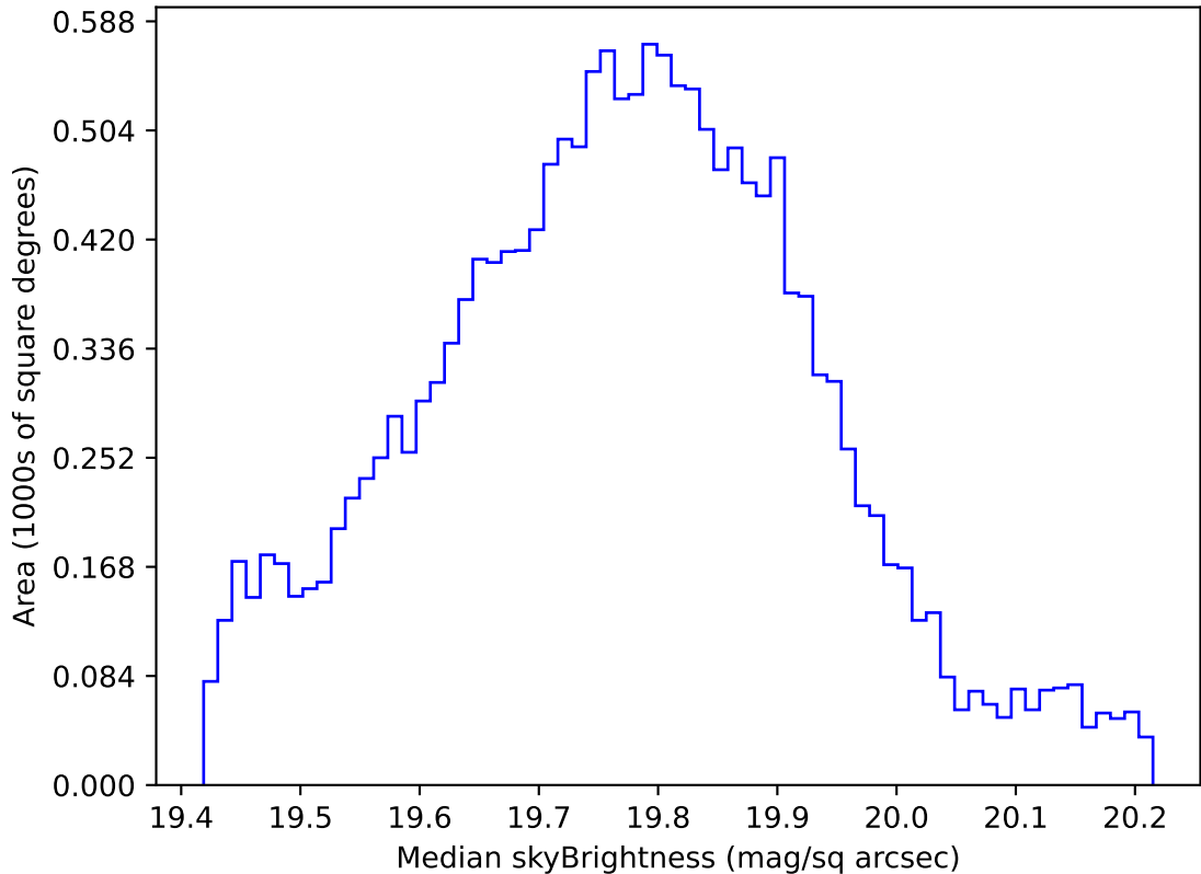
internal_u_expt30_nscale1.0v3.4_10yrs WFD all bands: Median skyBrightness
