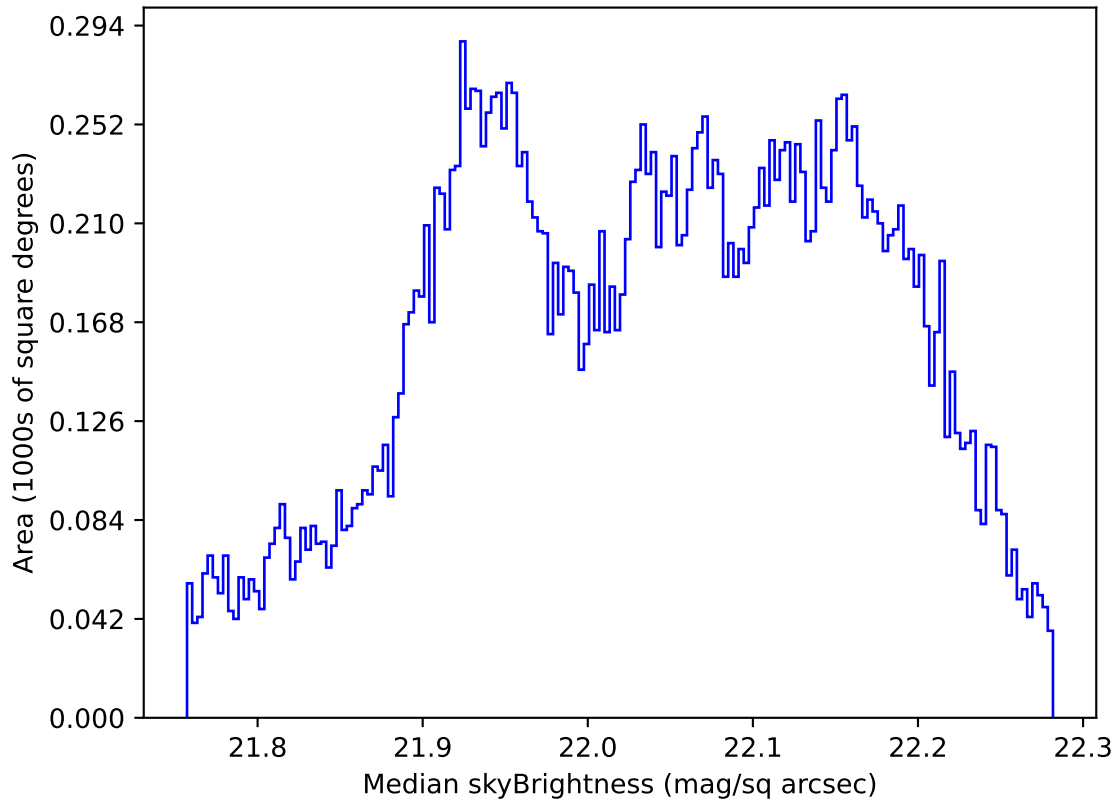
internal_u_expt30_nscale1.0v3.4_10yrs All sky g band: Median skyBrightness
