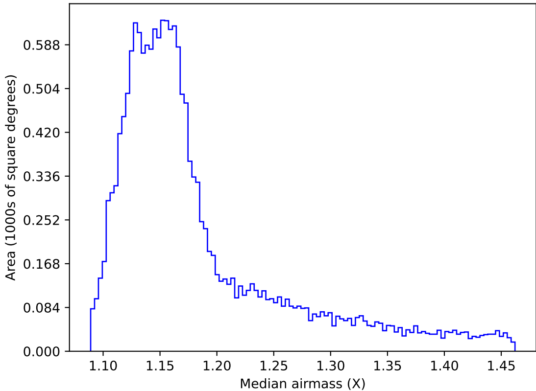
internal_u_expt30_nscale1.0v3.4_10yrs WFD z band: Median airmass
