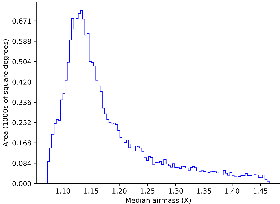
internal_u_expt30_nscale1.0v3.4_10yrs WFD u band: Median airmass
