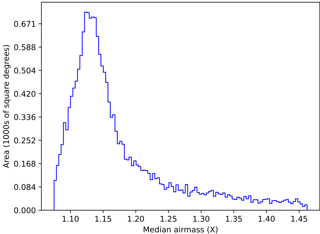
internal_u_expt30_nscale1.0v3.4_10yrs WFD r band: Median airmass
