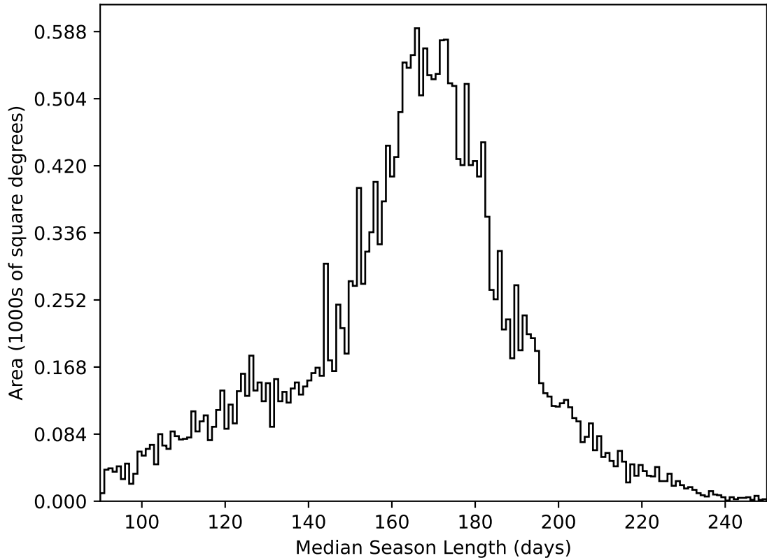
internal_u_expt30_nscale1.0v3.4_10yrs All sky all bands: Median Season Length
