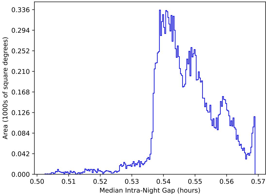
internal_u_expt30_nscale1.0v3.4_10yrs WFD: Median Intra-Night Gap
