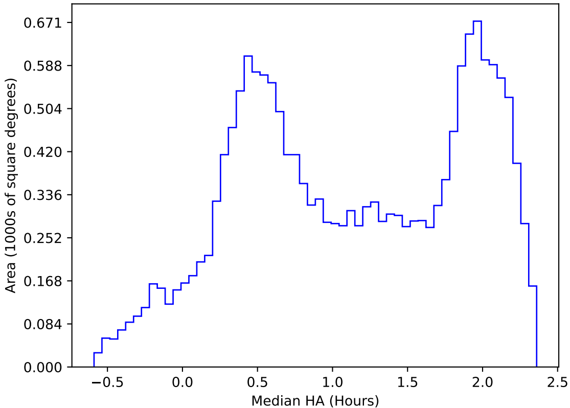
internal_u_expt30_nscale1.0v3.4_10yrs WFD z band: Median HA
