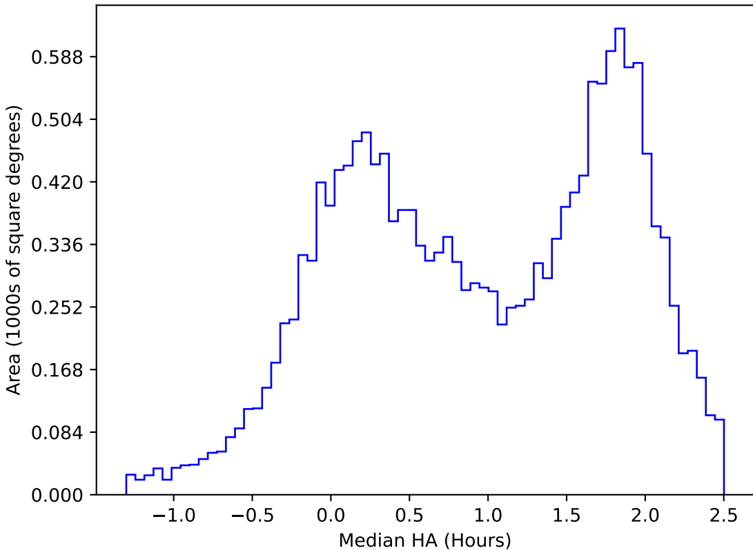
internal_u_expt30_nscale1.0v3.4_10yrs WFD u band: Median HA
