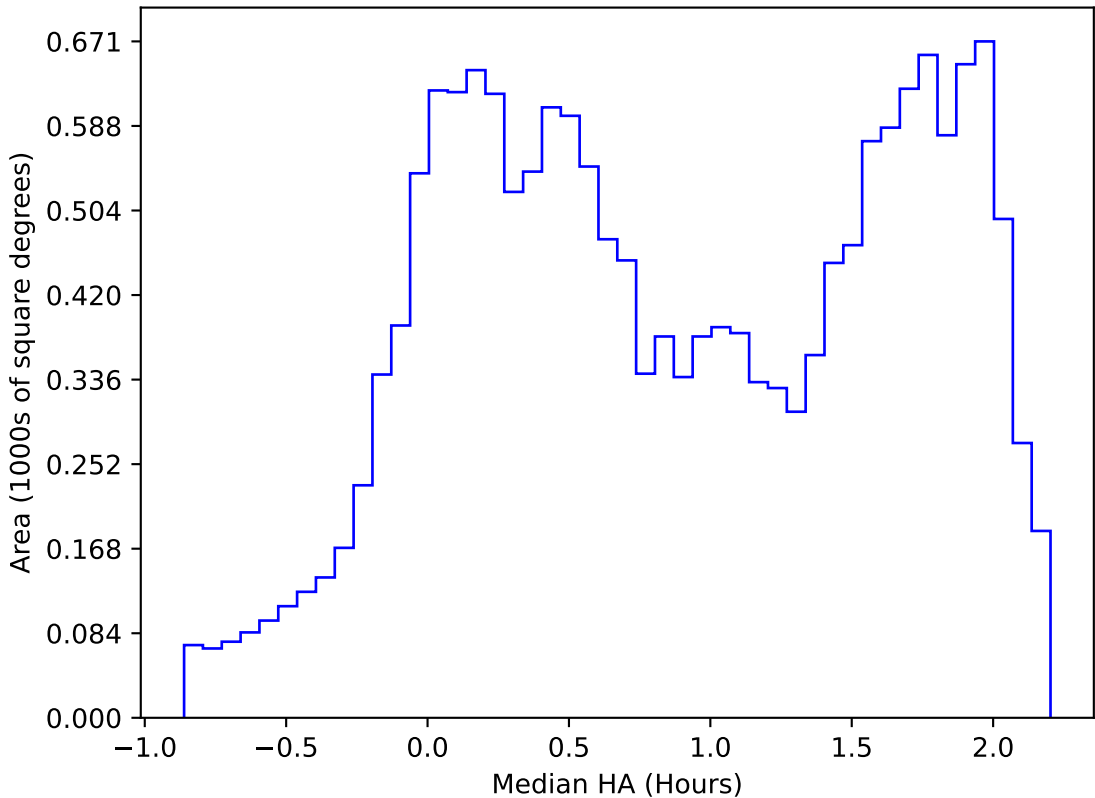
internal_u_expt30_nscale1.0v3.4_10yrs WFD r band: Median HA
