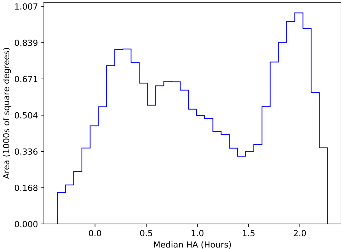
internal_u_expt30_nscale1.0v3.4_10yrs WFD i band: Median HA
