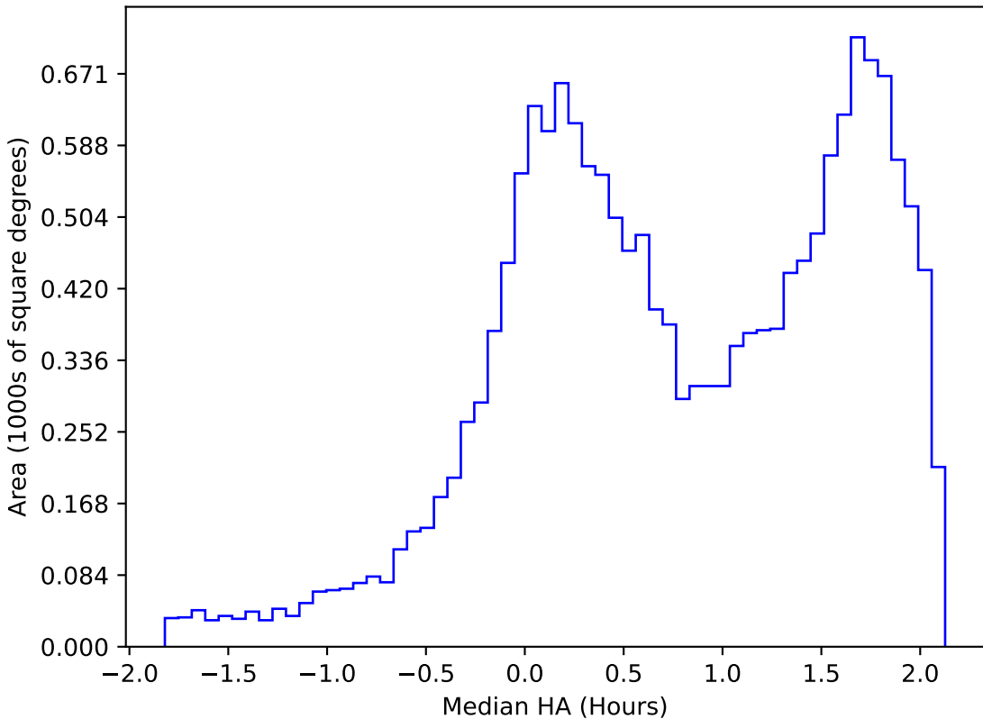
internal_u_expt30_nscale1.0v3.4_10yrs WFD g band: Median HA
