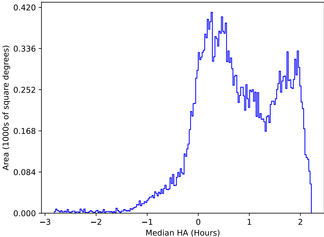
internal_u_expt30_nscale1.0v3.4_10yrs All sky r band: Median HA
