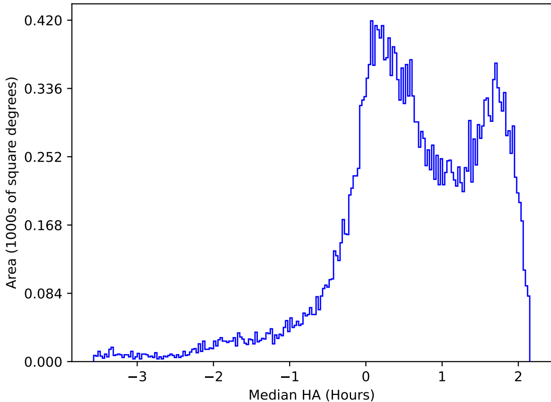
internal_u_expt30_nscale1.0v3.4_10yrs All sky g band: Median HA
