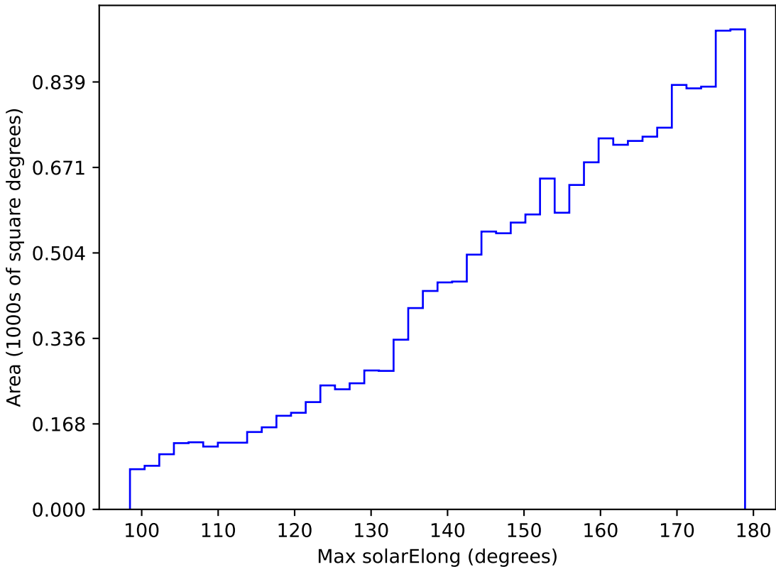
internal_u_expt30_nscale1.0v3.4_10yrs WFD g band: Max solarElong
