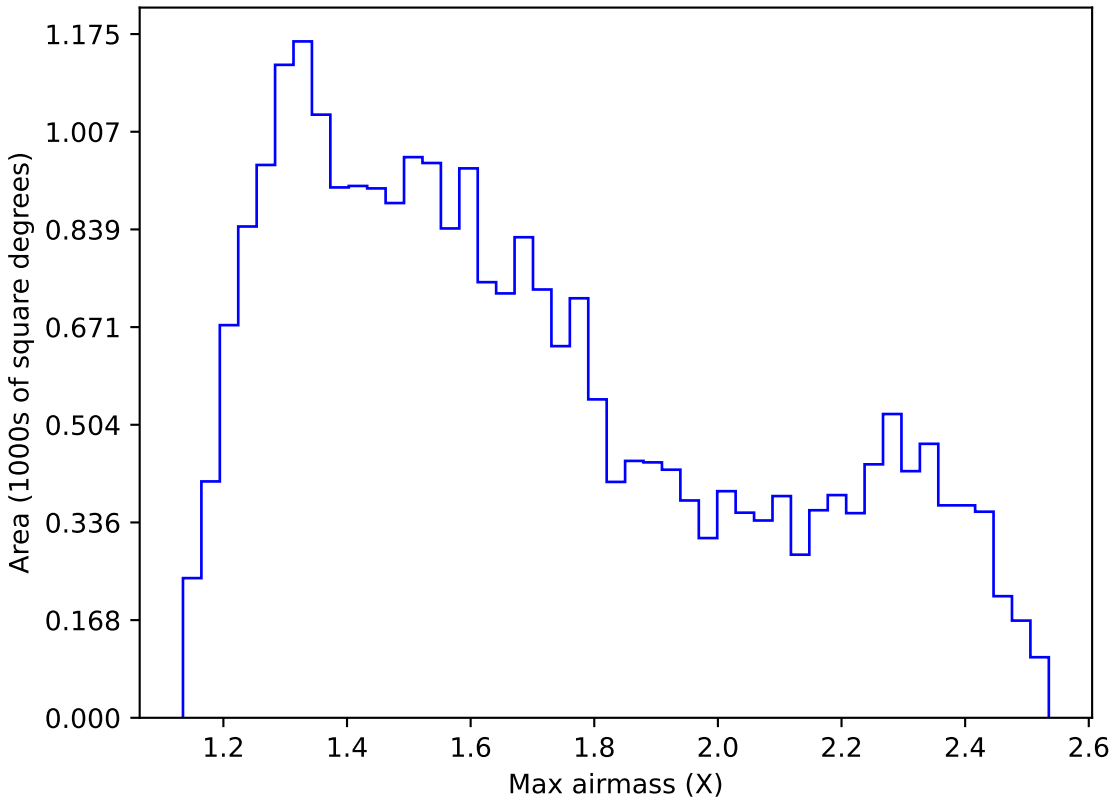
internal_u_expt30_nscale1.0v3.4_10yrs Yr 1 r band: Max airmass
