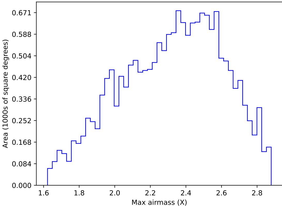
internal_u_expt30_nscale1.0v3.4_10yrs WFD y band: Max airmass
