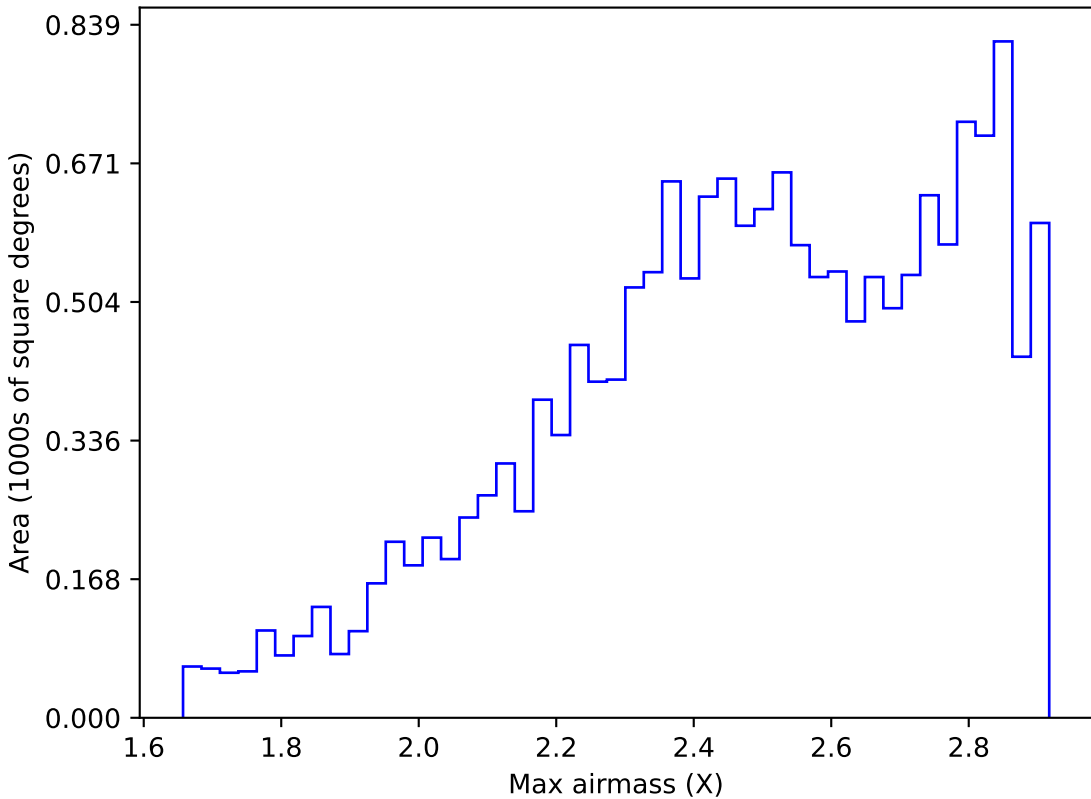
internal_u_expt30_nscale1.0v3.4_10yrs WFD i band: Max airmass
