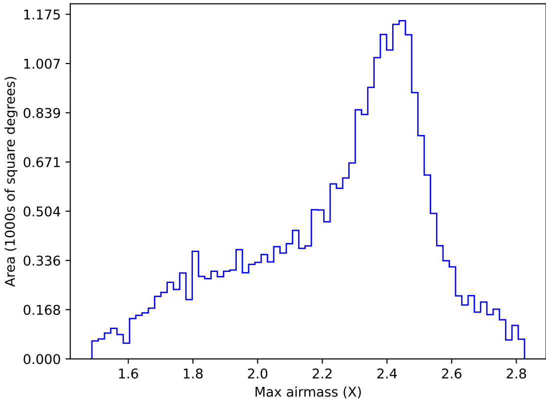
internal_u_expt30_nscale1.0v3.4_10yrs All sky r band: Max airmass
