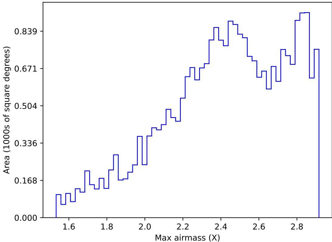
internal_u_expt30_nscale1.0v3.4_10yrs All sky i band: Max airmass
