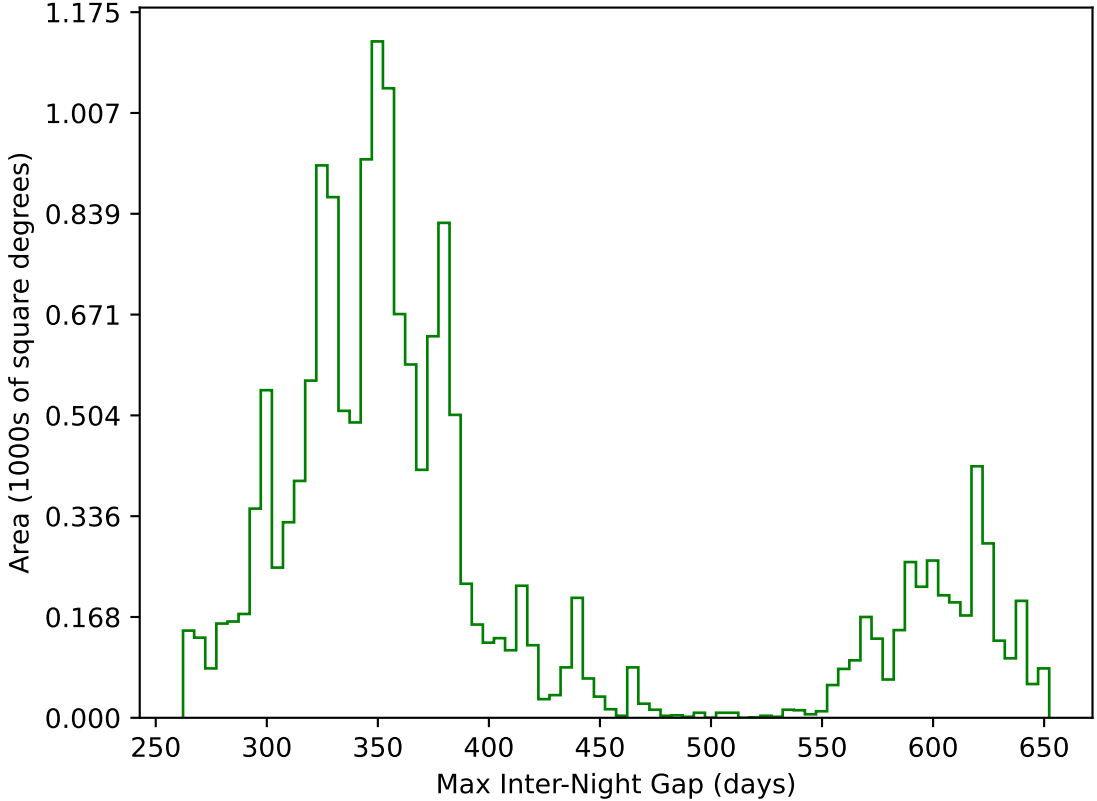
internal_u_expt30_nscale1.0v3.4_10yrs WFD g band: Max Inter-Night Gap
