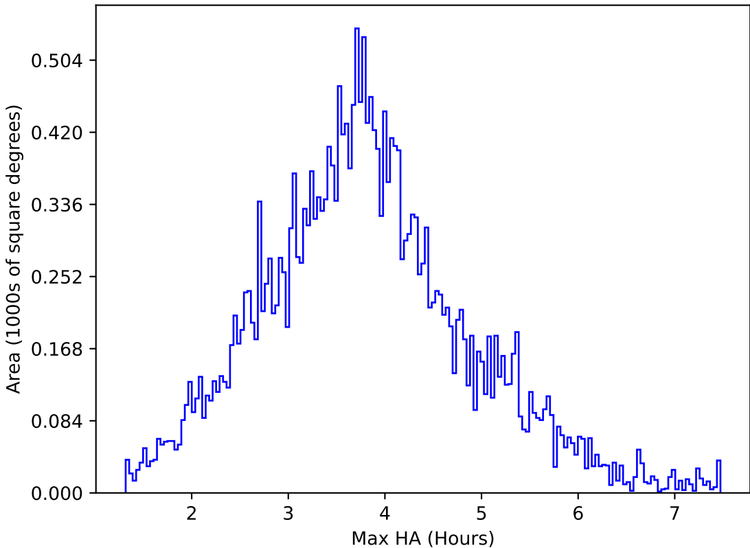
internal_u_expt30_nscale1.0v3.4_10yrs All sky g band: Max HA
