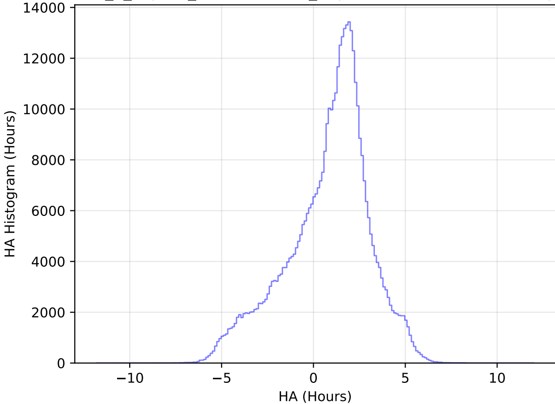
internal_u_expt30_nscale1.0v3.4_10yrs WFD z band: HA Histogram
