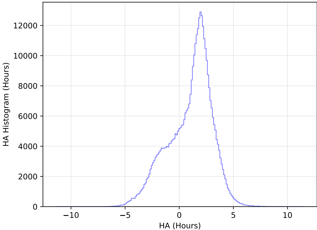
internal_u_expt30_nscale1.0v3.4_10yrs WFD y band: HA Histogram
