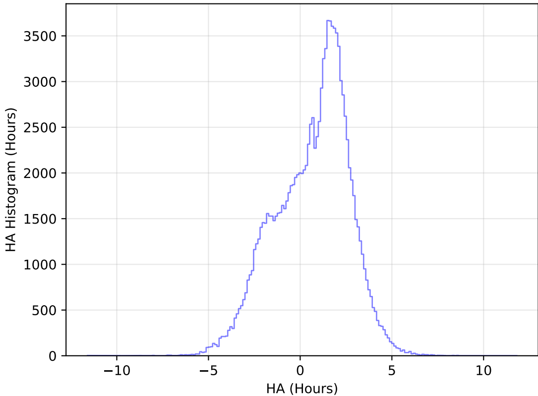
internal_u_expt30_nscale1.0v3.4_10yrs WFD u band: HA Histogram
