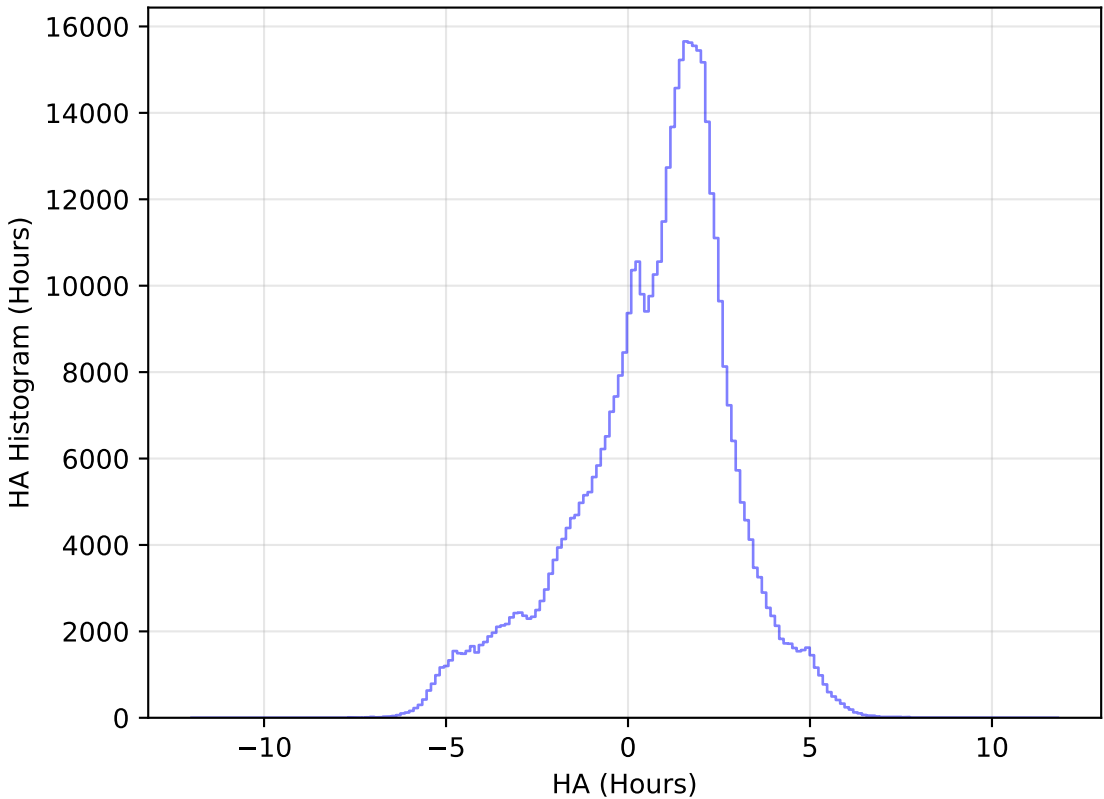
internal_u_expt30_nscale1.0v3.4_10yrs WFD i band: HA Histogram
