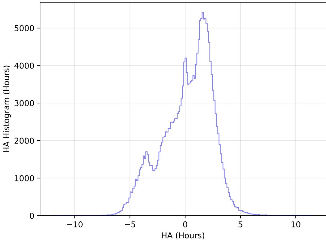
internal_u_expt30_nscale1.0v3.4_10yrs WFD g band: HA Histogram
