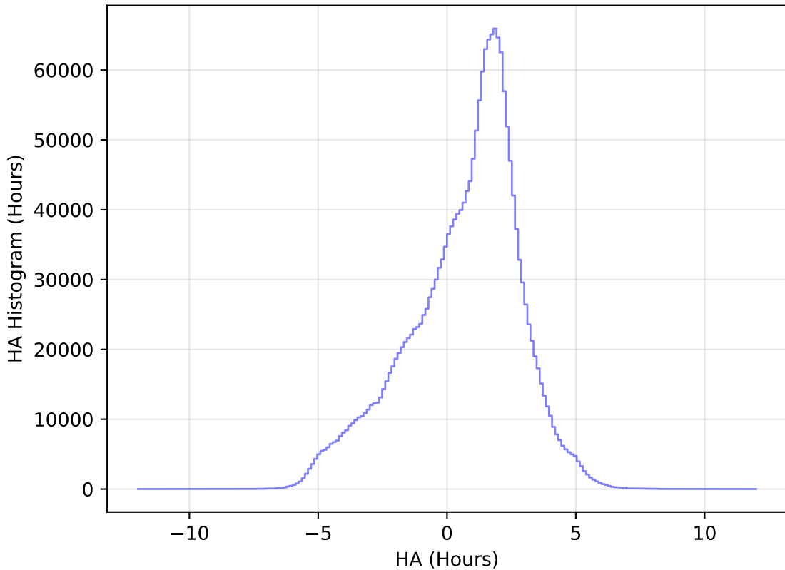
internal_u_expt30_nscale1.0v3.4_10yrs WFD all bands: HA Histogram
