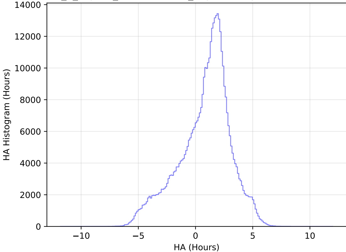
internal_u_expt30_nscale1.0v3.4_10yrs All sky z band: HA Histogram
