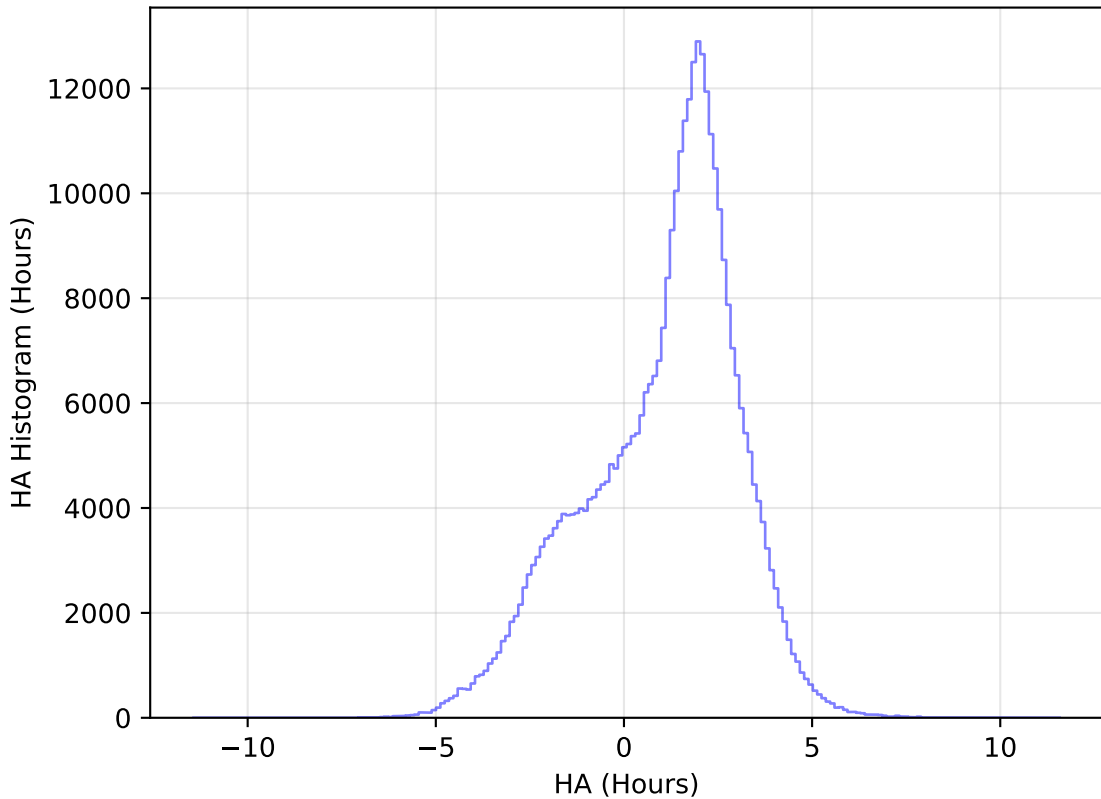
internal_u_expt30_nscale1.0v3.4_10yrs All sky y band: HA Histogram
