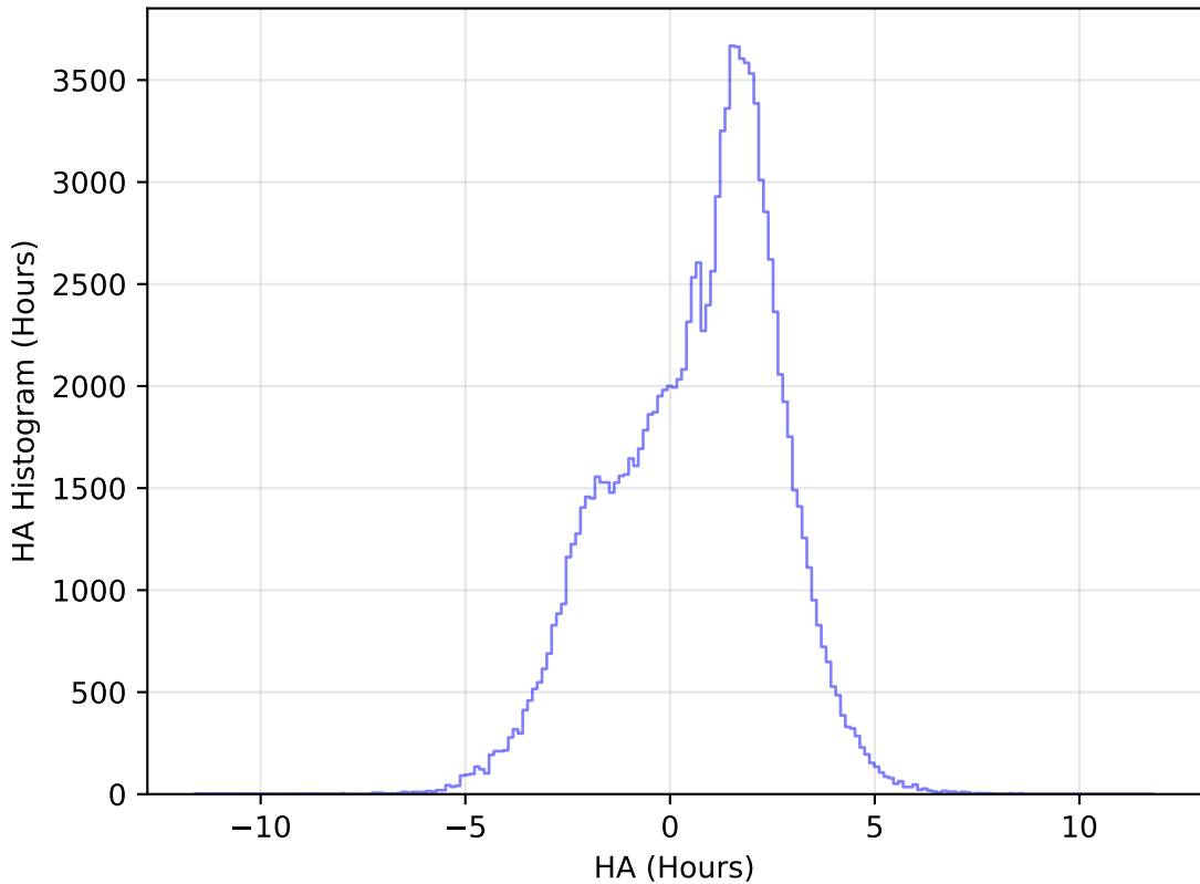
internal_u_expt30_nscale1.0v3.4_10yrs All sky u band: HA Histogram
