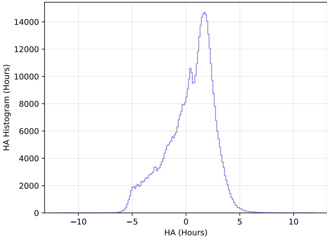
internal_u_expt30_nscale1.0v3.4_10yrs All sky r band: HA Histogram
