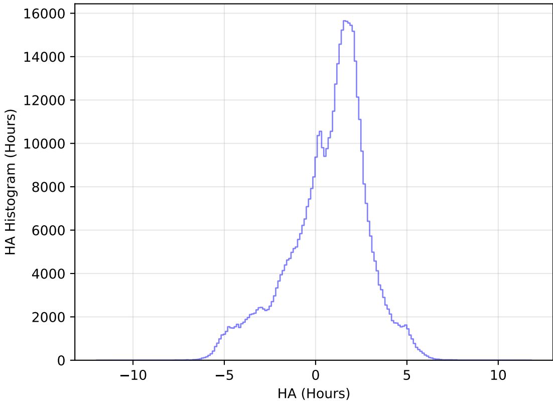
internal_u_expt30_nscale1.0v3.4_10yrs All sky i band: HA Histogram
