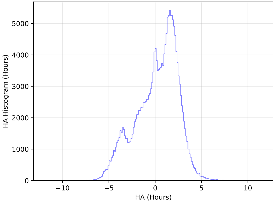
internal_u_expt30_nscale1.0v3.4_10yrs All sky g band: HA Histogram
