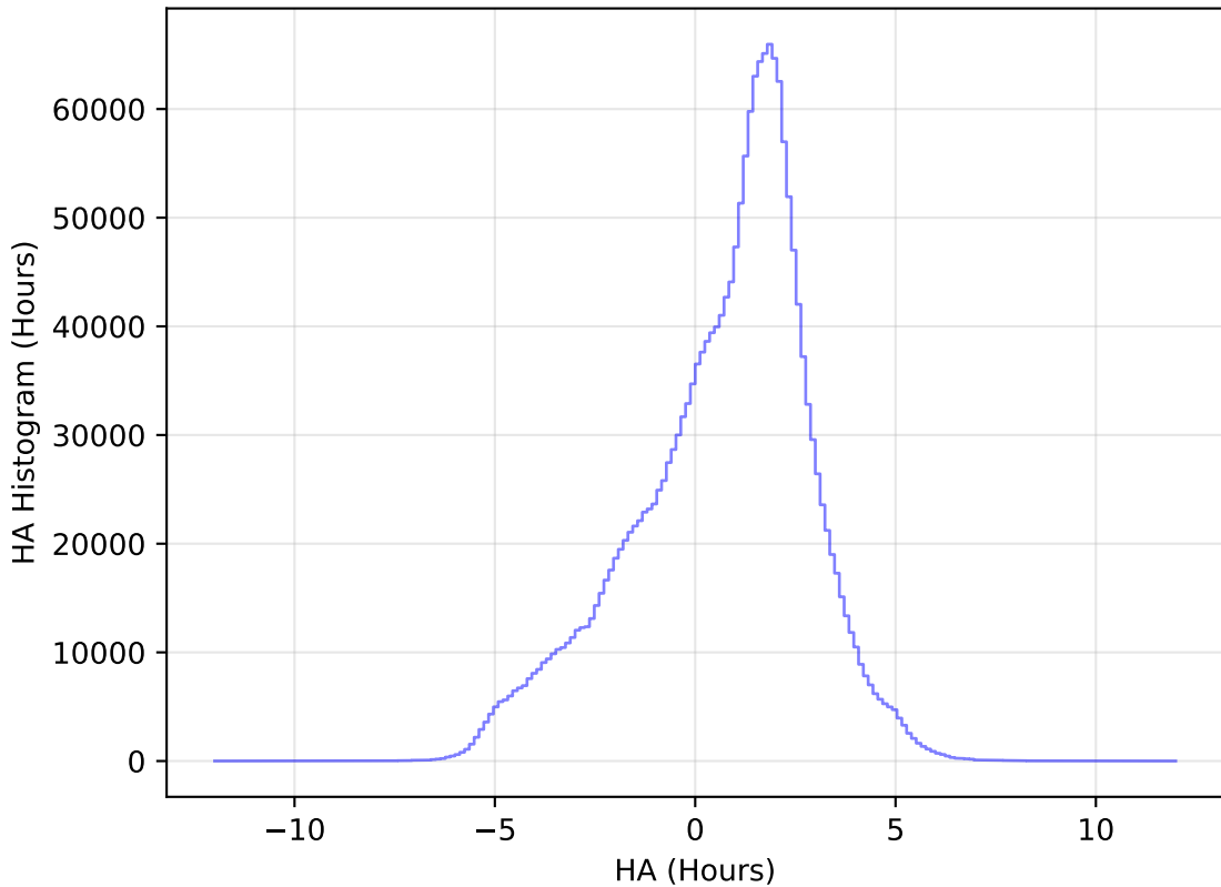
internal_u_expt30_nscale1.0v3.4_10yrs All sky all bands: HA Histogram
